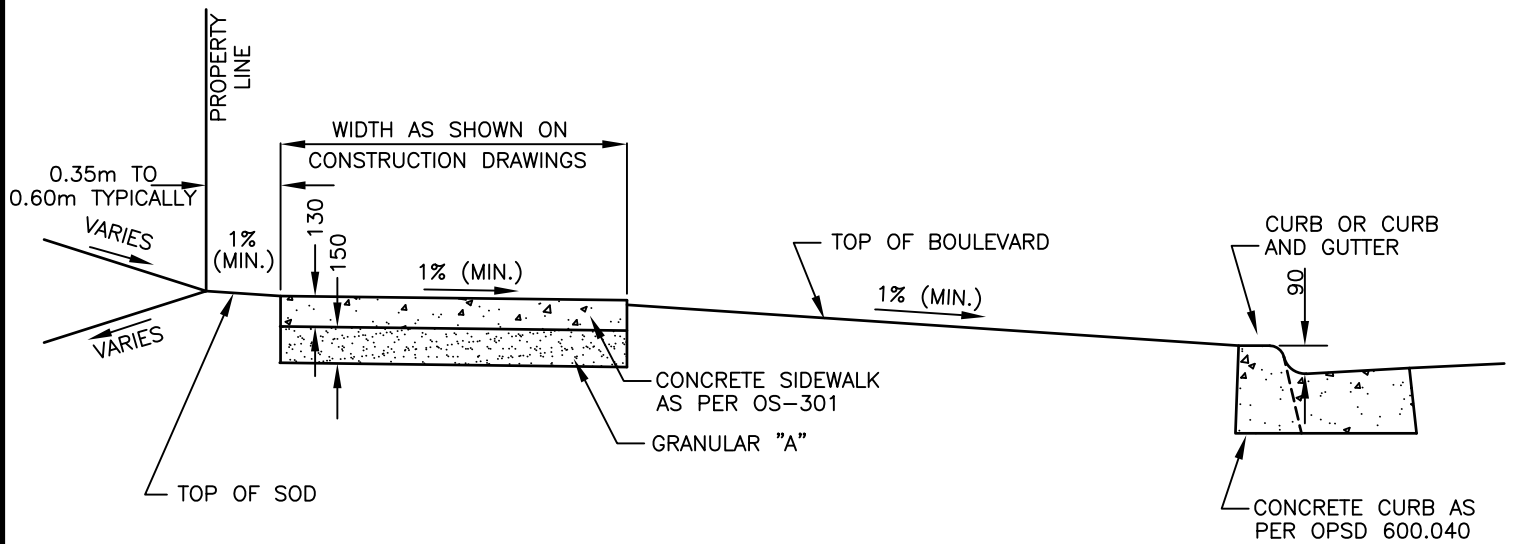
TYPICAL OVERLAND FLOW OUTLET
