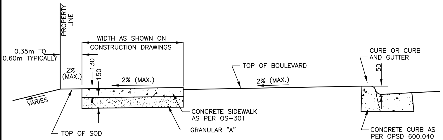
REVERSE SLOPE OVERLAND FLOW OUTLET
