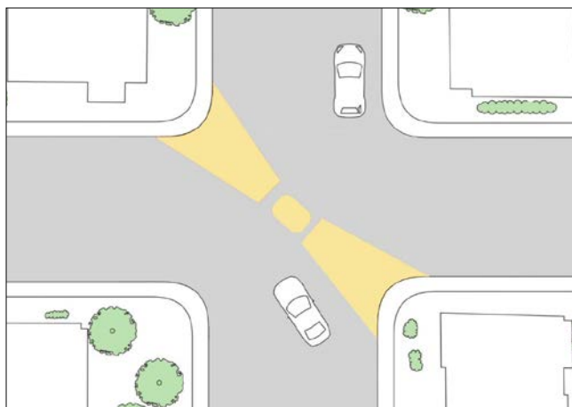
Rendering demonstrating diverter
