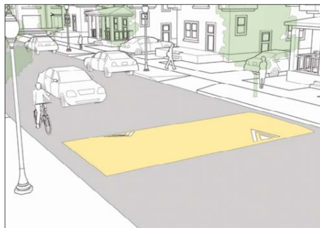
N.A.C.T.O. rendering of speed hump
