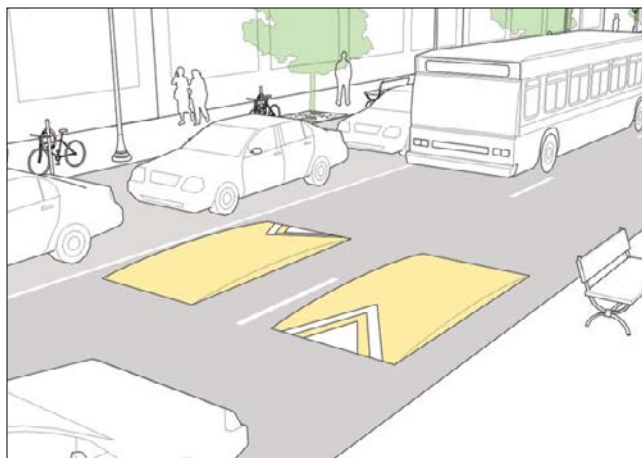
N.A.C.T.O. rendering of speed cushions
