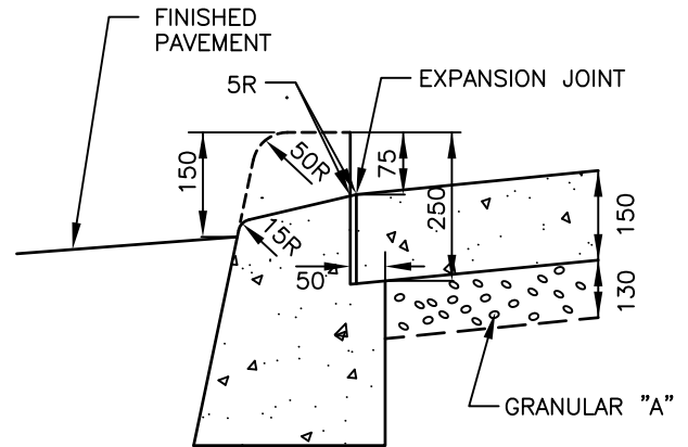
CURB DETAIL IN DRIVEWAY
