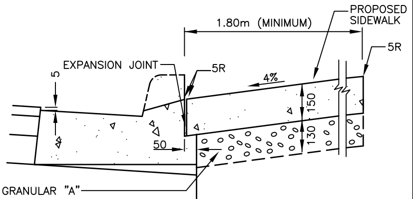
CROSS SECTION AT DRIVEWAY
