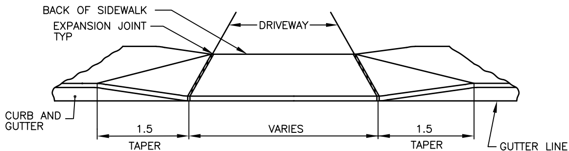
DRIVEWAY ELEVATION
